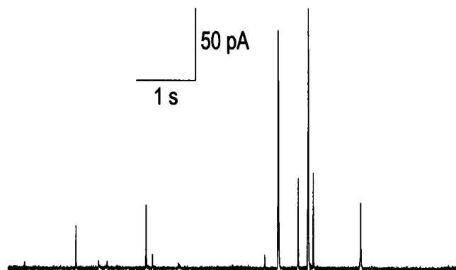
FIGURE 2 Single secretory events recorded at the surface of a chromaffin cell. Amperometric detection of exocytotic events induced by pressure ejection of 2 mM \text{Ba}^{2+} for 5 s.
