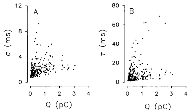
FIGURE 4 The kinetic parameters \sigma and \tau show little correlation with the integrated current ( Q ) of the spike. (A) Plot of \sigma versus Q . (B) Plot of \tau versus Q . The same 223 spikes presented in Fig. 3 B were analyzed.
